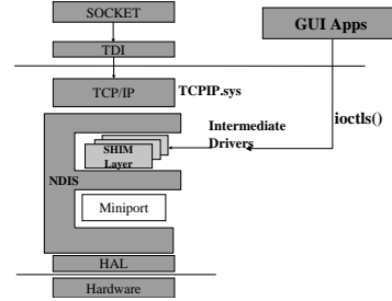
Figure 12: Windows intermediate driver architecture
